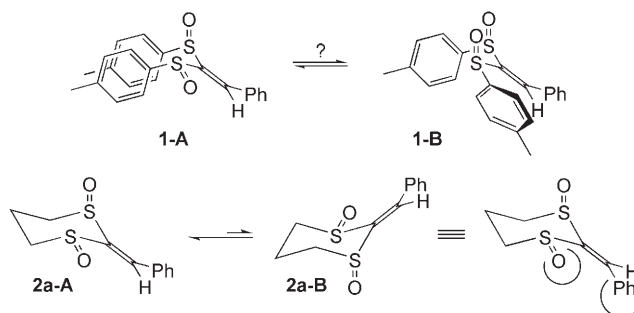
Scheme 2. Conformations in alkylidene bis(sulfoxides).
