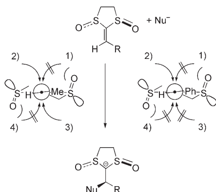
Scheme 6. Nucleophilic attack to dithiolane-derived alkylidene bis(sulfoxides). See text for details.
