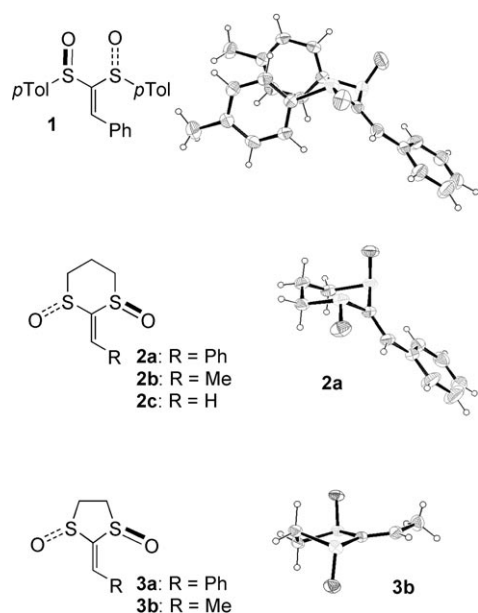
Figure 1. Alkylidene bis(sulfoxides) and their crystal structures. [7] top; [11a] middle; [5] bottom. [6]
