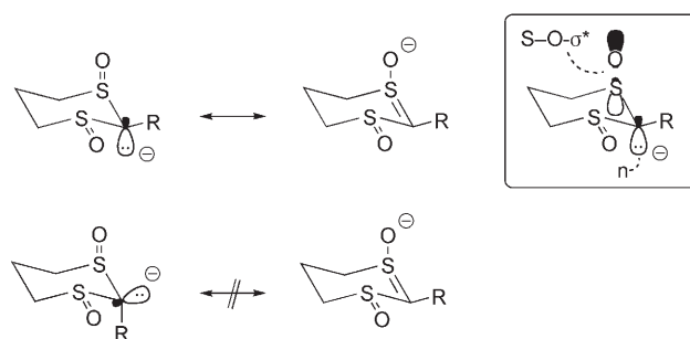
Figure 2. Stereoelectronic effects in sulfinyl carbanions.
