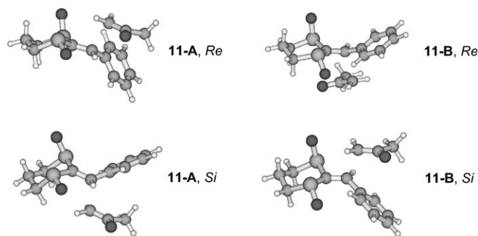
Figure 3. Calculated transition states for attack of acetone enolate to alkylidene bis(sulfoxide) 2a . [7]
