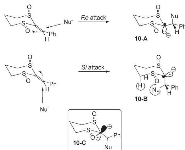
Scheme 3. Carbanion formation through nucleophilic attack to alkylidene bis(sulfoxides).
