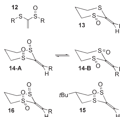
Figure 4. Sulfinylmethyl sulfides and axially chiral bis(sulfoxides).
