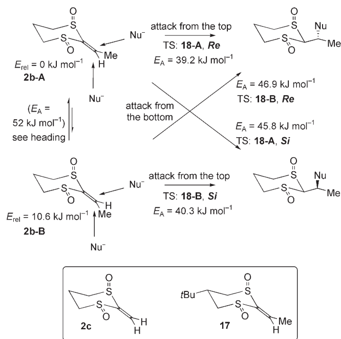
Scheme 4. Nucleophilic attacks to substrates bearing a small methyl group ( \text{Nu}^- = acetone enolate). All values were calculated (BP86/aug-TZVP) except for the activation barrier for the conformational interchange between 2b-A and 2b-B which was measured by NMR spectroscopy for the parent compound 2c .
